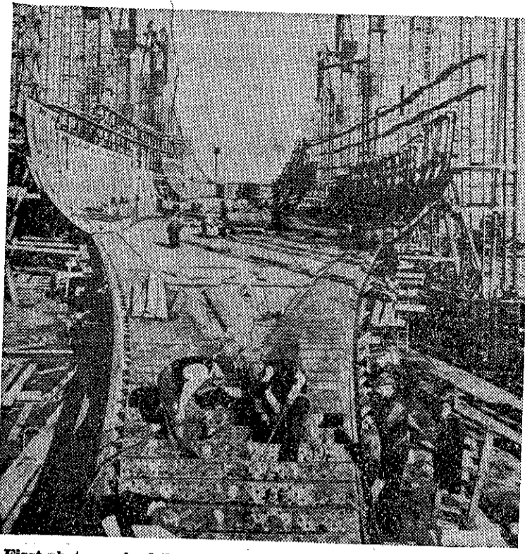
First photograph of the new 32,000-ton Cunard White Star liner, as yet known only as No. 1029, shows a view of the hull skeleton, looking toward the stern on the stocks of the shipyard at Birkenhead, England. This is the largest ship ever laid down in England.
