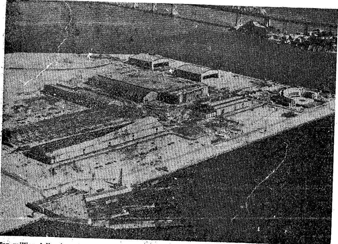
Ten million dollars' worth of buildings for the 1939 Golden Gate International exposition are already under construction on Treasure island in San Francisco bay site of the fair. Photograph shows the latest air view of the exposition grounds. In the foreground are the ferry slips and ferry terminal designed to handle the peak world's fair crowds of 40,000 persons an hour.
