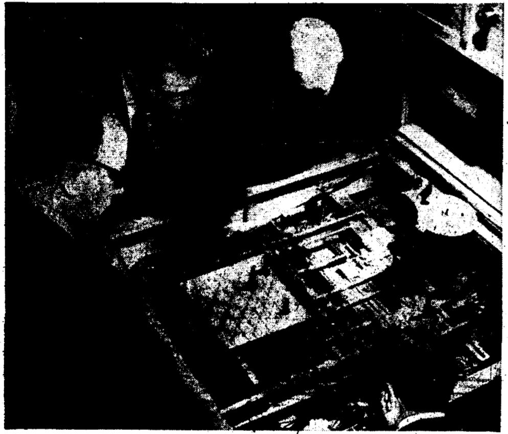
ELECTRIC CHESS-PLAYING machine is studied in action by Leonardo Torres-Quevedo (right background) and French engineers in Paris. Machine's play is limited to rook and king against king, but it invariably brings off the mate. If the human player cheats or makes an error, the machine signals and waits until move has been corrected before continuing.
