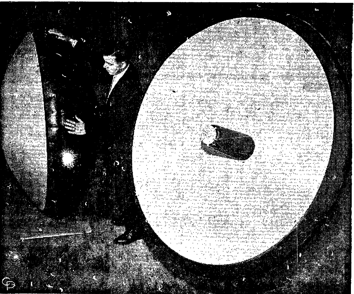
"INSTANT ANTENNA" —These inflatable antennas, shown at Goodyear Aerospace in Akron, O., are test models fabricated for the U.S. Army Electronics Command, Fort Monmouth, N.J., which wants such antennas for use by highly mobile forces. They can be inflated or folded for use again in a matter of minutes.
