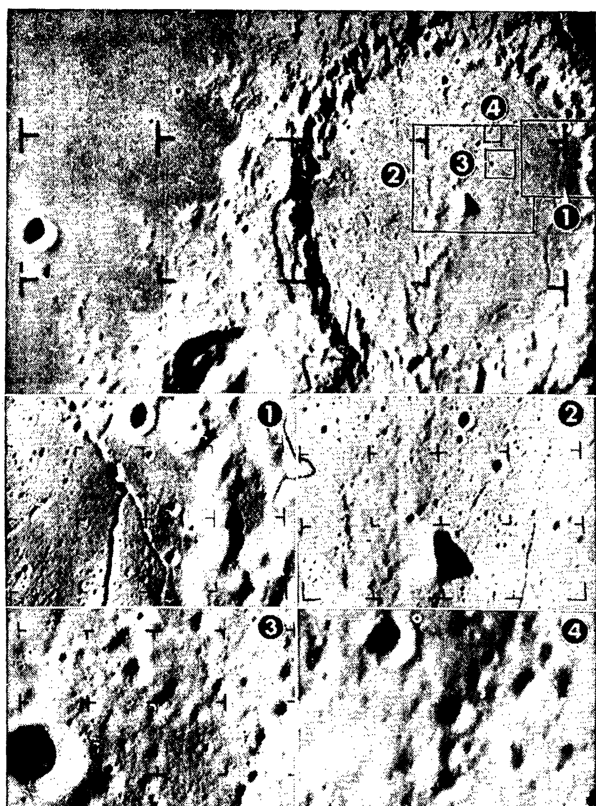
DETAILED STUDY of the Moon photos televised by Ranger-9 brings out these interesting comparisons. Top: The crater Alphonsus from 258 miles away. Smaller crater at left is Alpetragius. Numbers on the boxes in Alphonsus correspond to the four photos below. No. 1, one minute, 17 seconds before impact. Eastern edge of crater is seen from 115 miles out. No. 2, at 38.8 seconds before impact, from 58 miles. No. 3, from 12.2 miles, 8.09 seconds before impact. No. 4, the last photo, from three-fourths of a mile, 0.463 seconds before impact. Small white circle at top is the point of impact.
